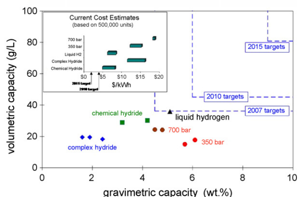
Fig. 2. Current status of hydrogen storage system capacity and cost [4].
