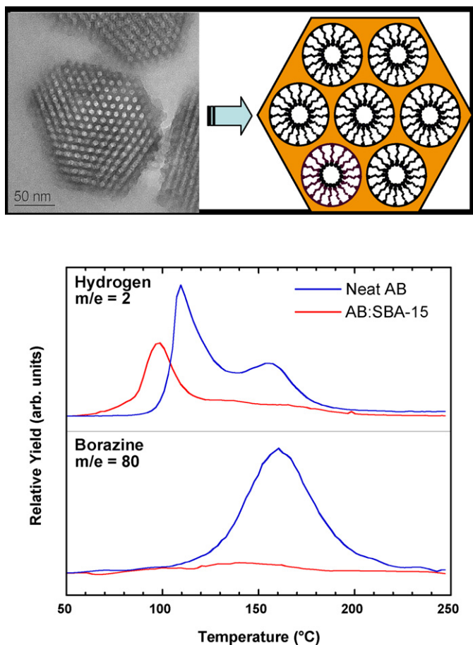
Fig. 9. Improved release of hydrogen from \text{NH}_3\text{BN}_3 via a mesoporous silica scaffold arrangement [4,31].
